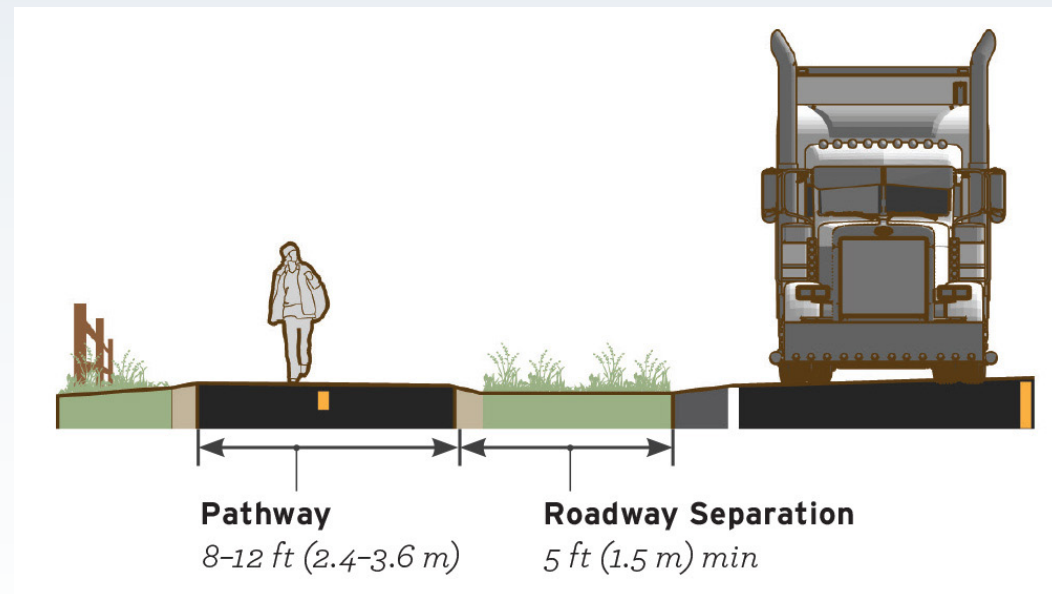
► Separated Path and Roadway
